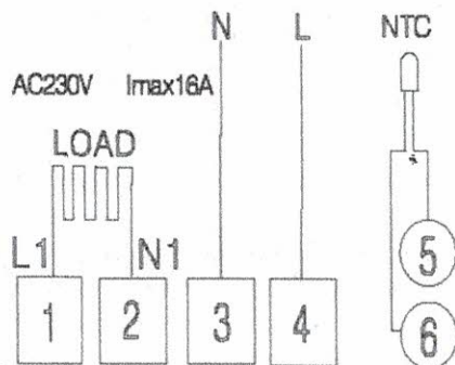
Electric heating wiring diagram
